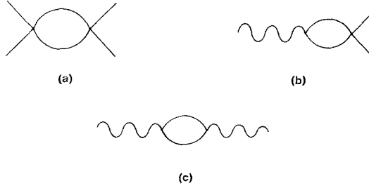
Fig. 1. Diagrams involved in the computation of the b , c_2 , and l functions in the one-loop approximation.
