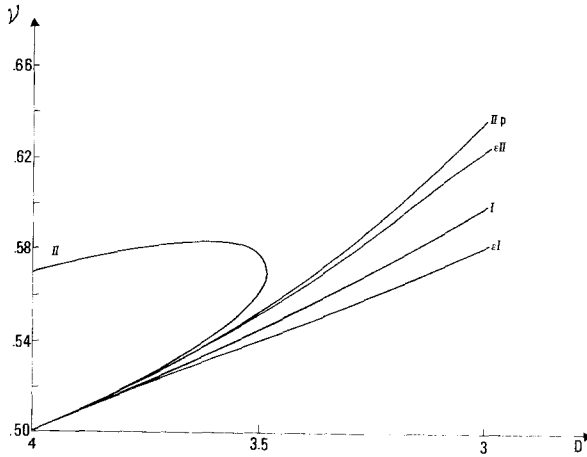
Fig. 3. Plot of the critical exponent \nu of the Ising model in different approximations: \epsilon I and \epsilon II are, respectively, the first and the second order in \epsilon ; I and II are the critical exponents produced respectively by the one-loop and the two-loop approximations using the g_c given by the Taylor expansion, while in IIP we use the g_c computed from the [2, 1] Padé approximant.
